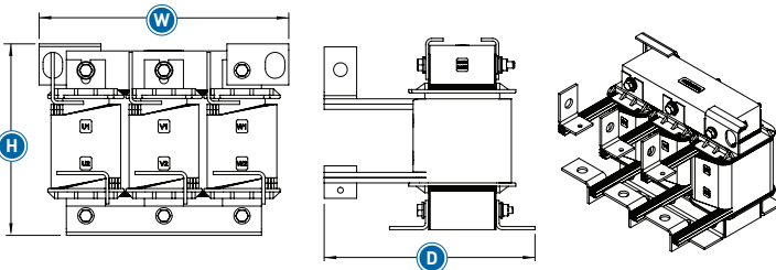
FIGURE 7 PANEL MOUNT
