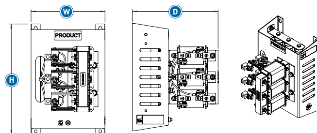
FIGURE 7 PANEL MOUNT
