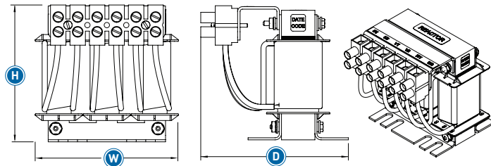
FIGURE 3 KIT
