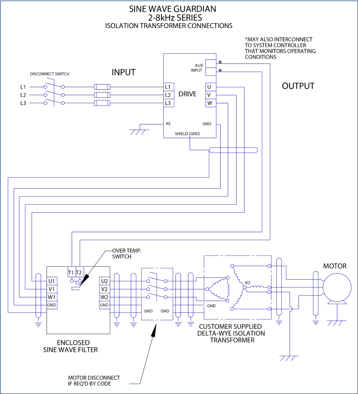
Figure 5-4: Isolation Transformer
