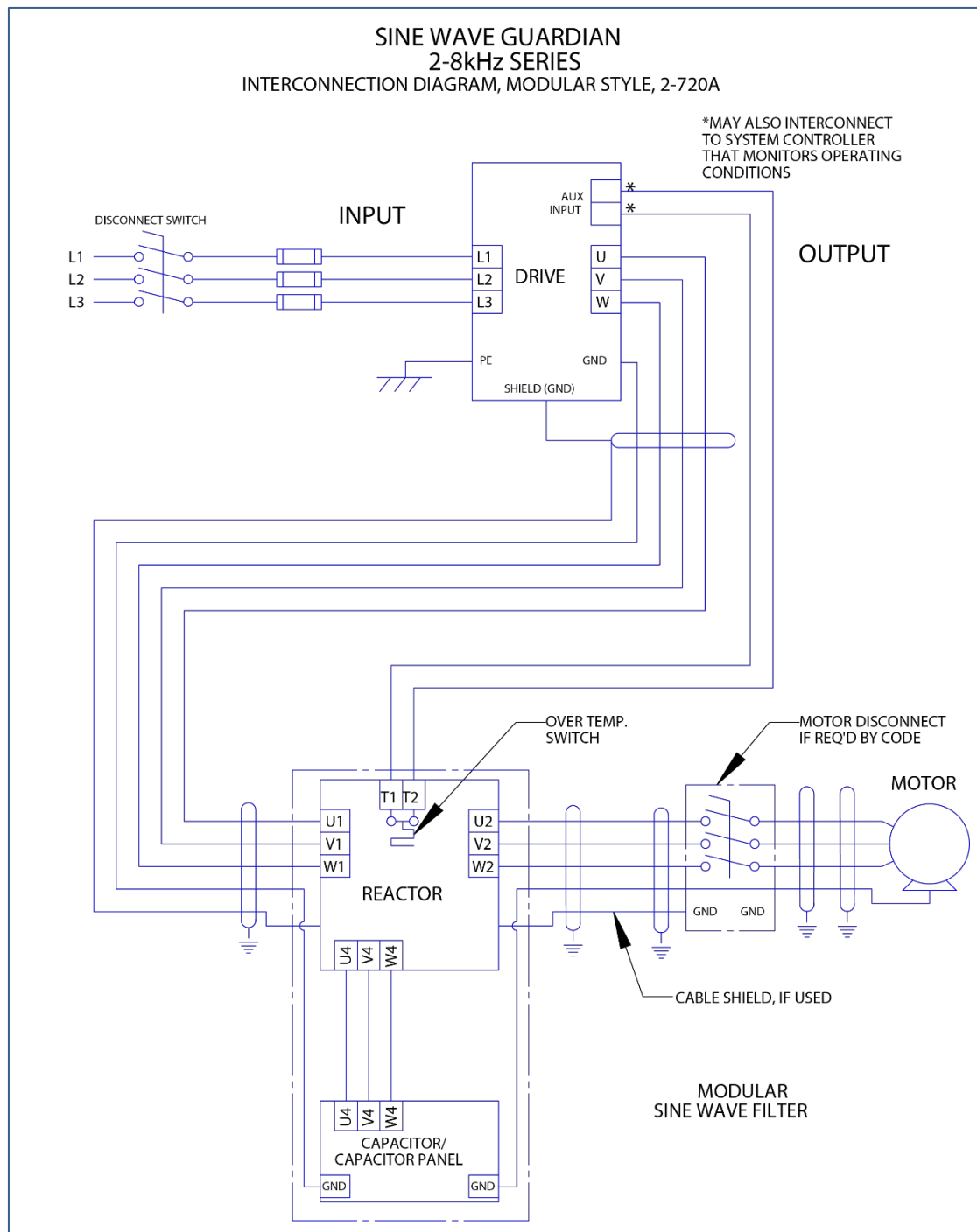
Figure 5-1: Modular Interconnection
